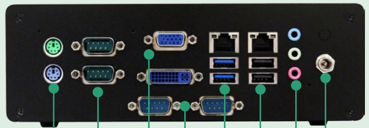
Rear I/O
